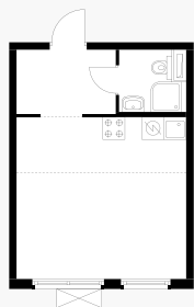
1NM1_4.8-1_S_A_4
